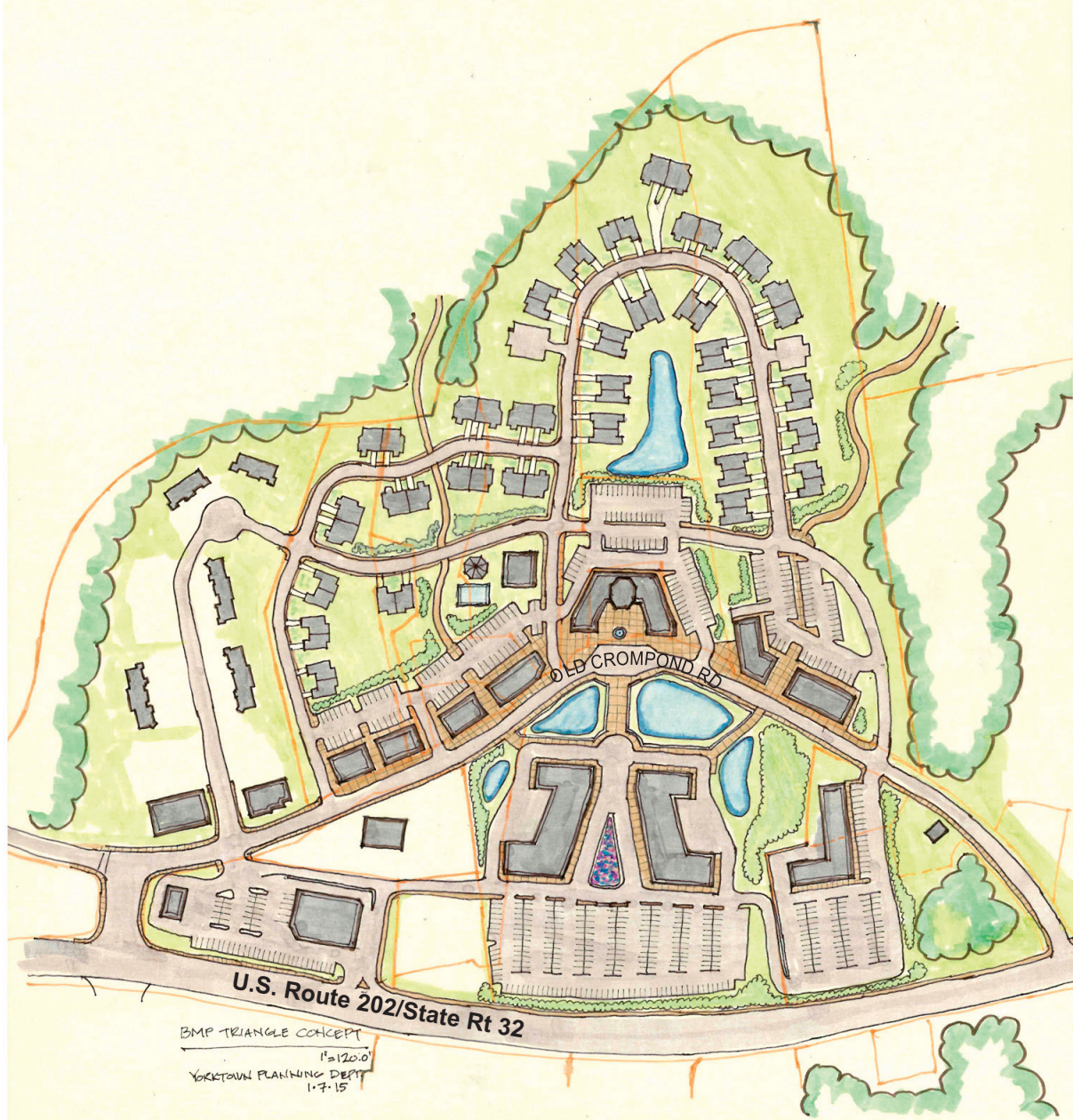
Figure 1-3: Conceptual Bear Mountain Triangle Master Plan Old Crompond Road, Town of Yorktown Westchester County, New York
